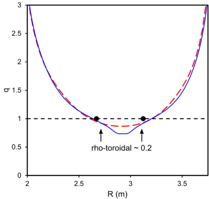
Figure 9. q -profiles from a TRANSP simulation (solid - blue) and EFIT constrained equilibrium reconstruction (broken - red) at t = 3.6 s for a protium plasma. Also shown is the inversion radius of the first sawtooth crash at t = 3.63 s (filled black circles) and the approximate location of \rho_{\text{tor}} = 0.2 .
